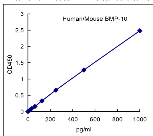
Plot Human/Mouse BMP-10 standard curve
