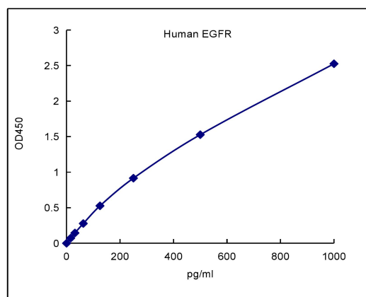
Plot Human EGFR standard curve
